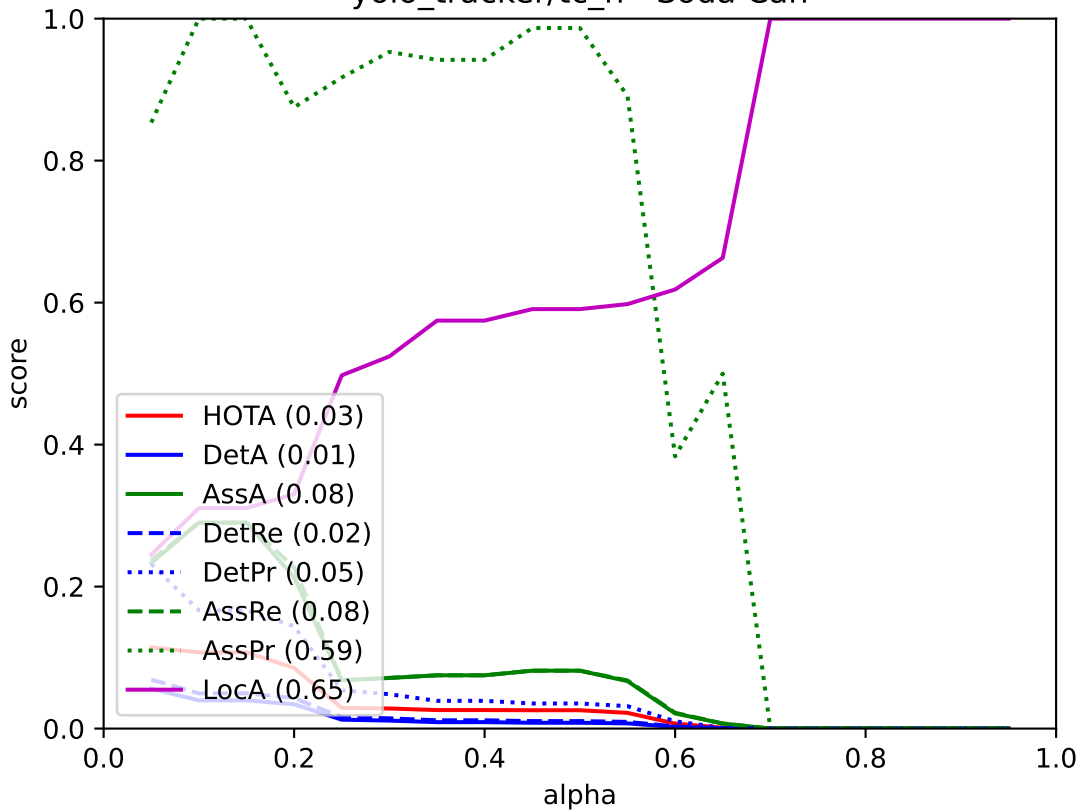
yolo_tracker/tc_n - Soda Can
